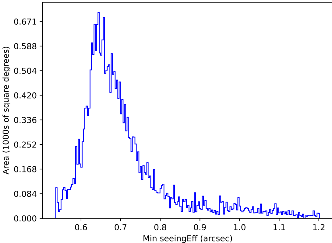
too_elab_r8_d2_gz_v3.4_10yrs Yr 1 i band: Min seeingEff
