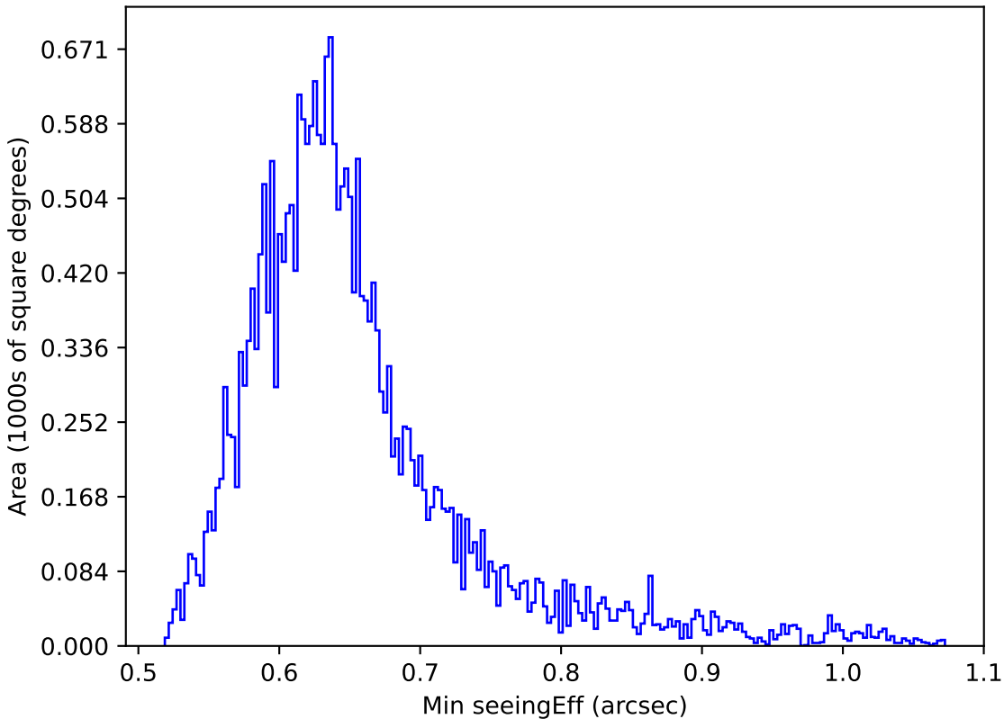
too_elab_r8_d2_gz_v3.4_10yrs Yr 1 all bands: Min seeingEff
