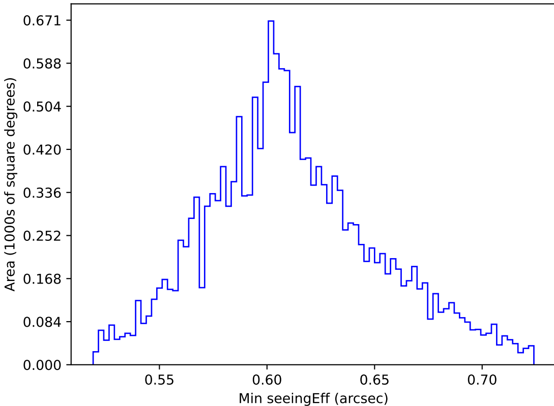
too_elab_r8_d2_gz_v3.4_10yrs WFD z band: Min seeingEff
