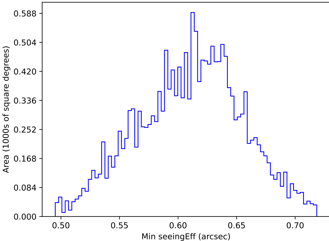
too_elab_r8_d2_gz_v3.4_10yrs WFD r band: Min seeingEff
