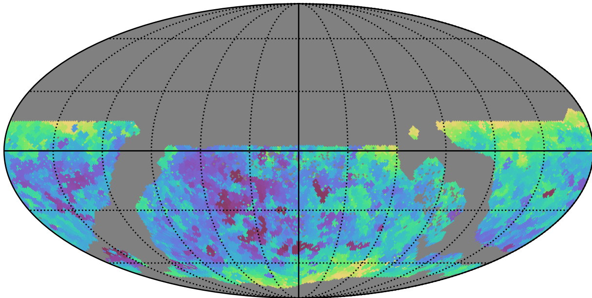
too_elab_r8_d2_gz_v3.4_10yrs WFD i band: Min seeingEff
