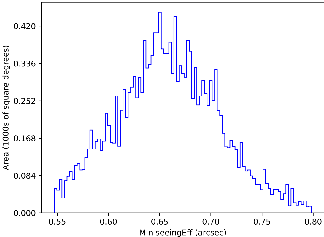
too_elab_r8_d2_gz_v3.4_10yrs WFD g band: Min seeingEff
