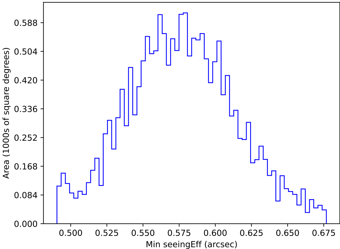
too_elab_r8_d2_gz_v3.4_10yrs WFD all bands: Min seeingEff
