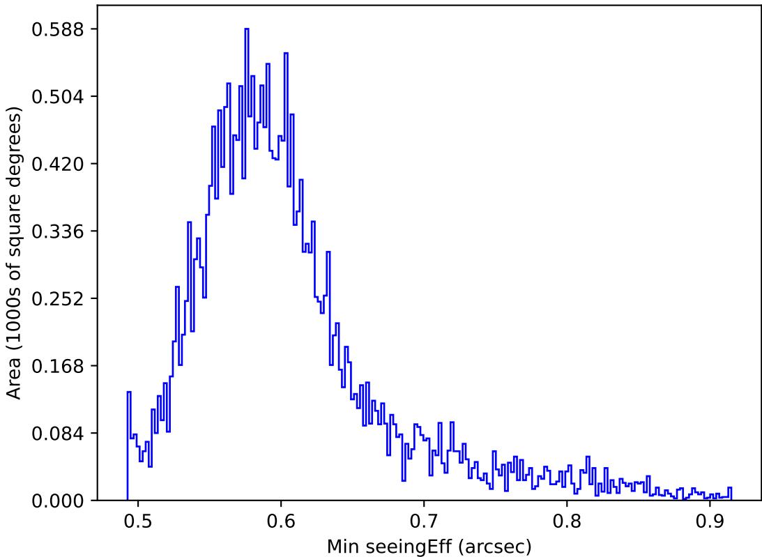
too_elab_r8_d2_gz_v3.4_10yrs All sky all bands: Min seeingEff
