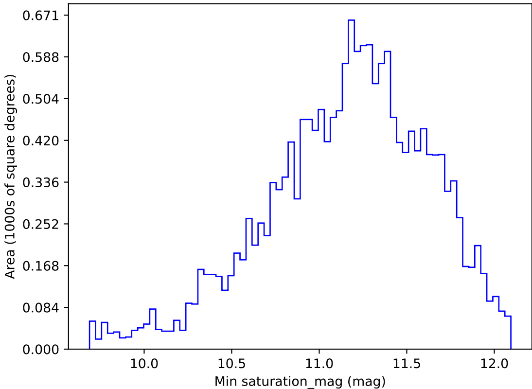
too_elab_r8_d2_gz_v3.4_10yrs WFD y band: Min saturation_mag
