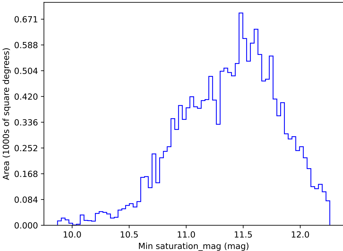
too_elab_r8_d2_gz_v3.4_10yrs WFD u band: Min saturation_mag
