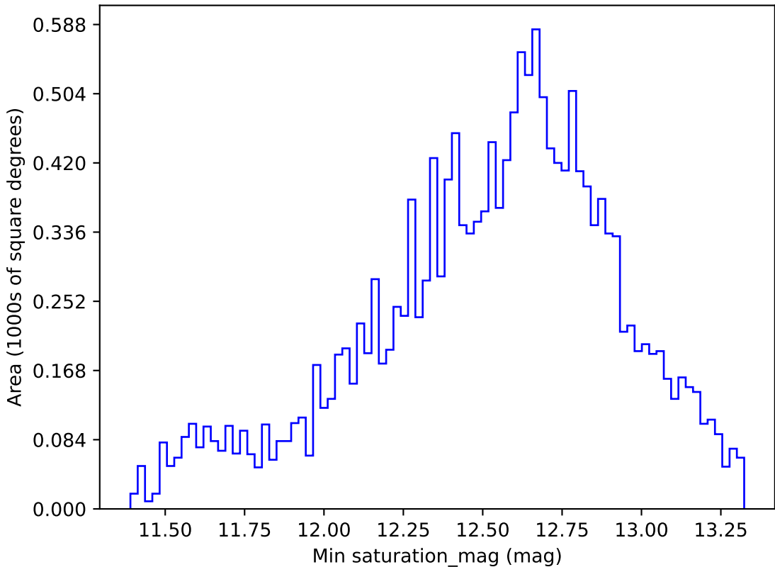
too_elab_r8_d2_gz_v3.4_10yrs WFD r band: Min saturation_mag
