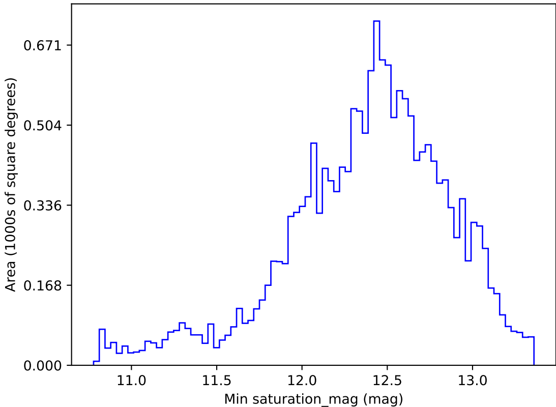
too_elab_r8_d2_gz_v3.4_10yrs WFD i band: Min saturation_mag
