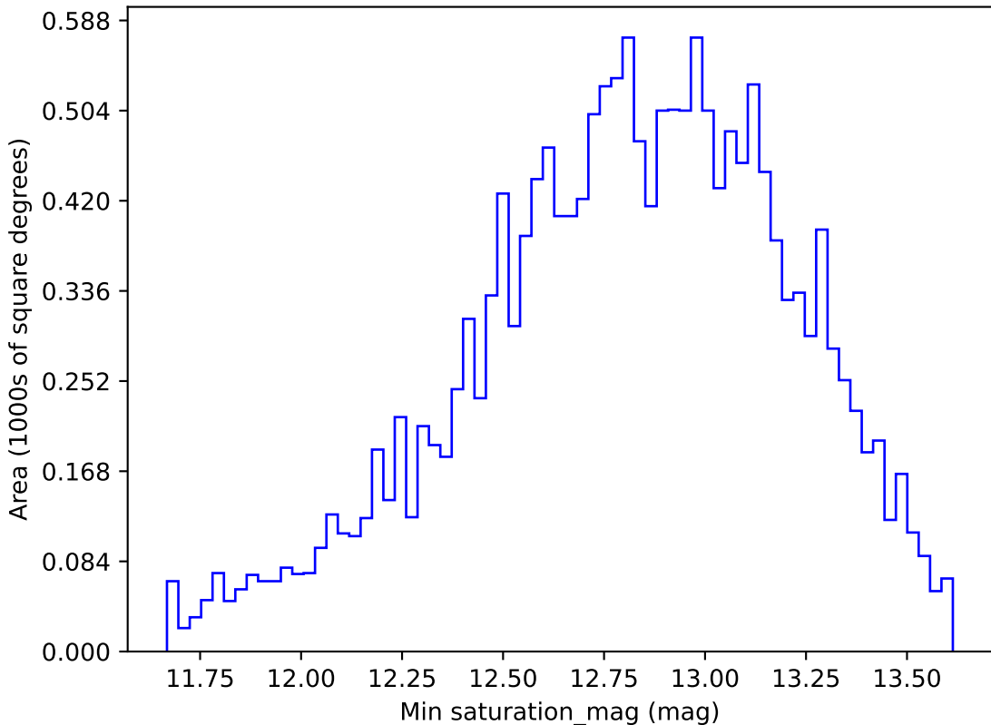
too_elab_r8_d2_gz_v3.4_10yrs WFD g band: Min saturation_mag
