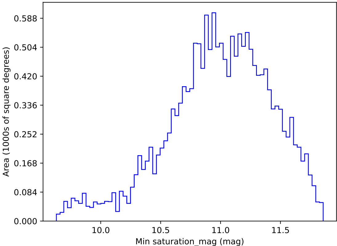
too_elab_r8_d2_gz_v3.4_10yrs WFD all bands: Min saturation_mag
