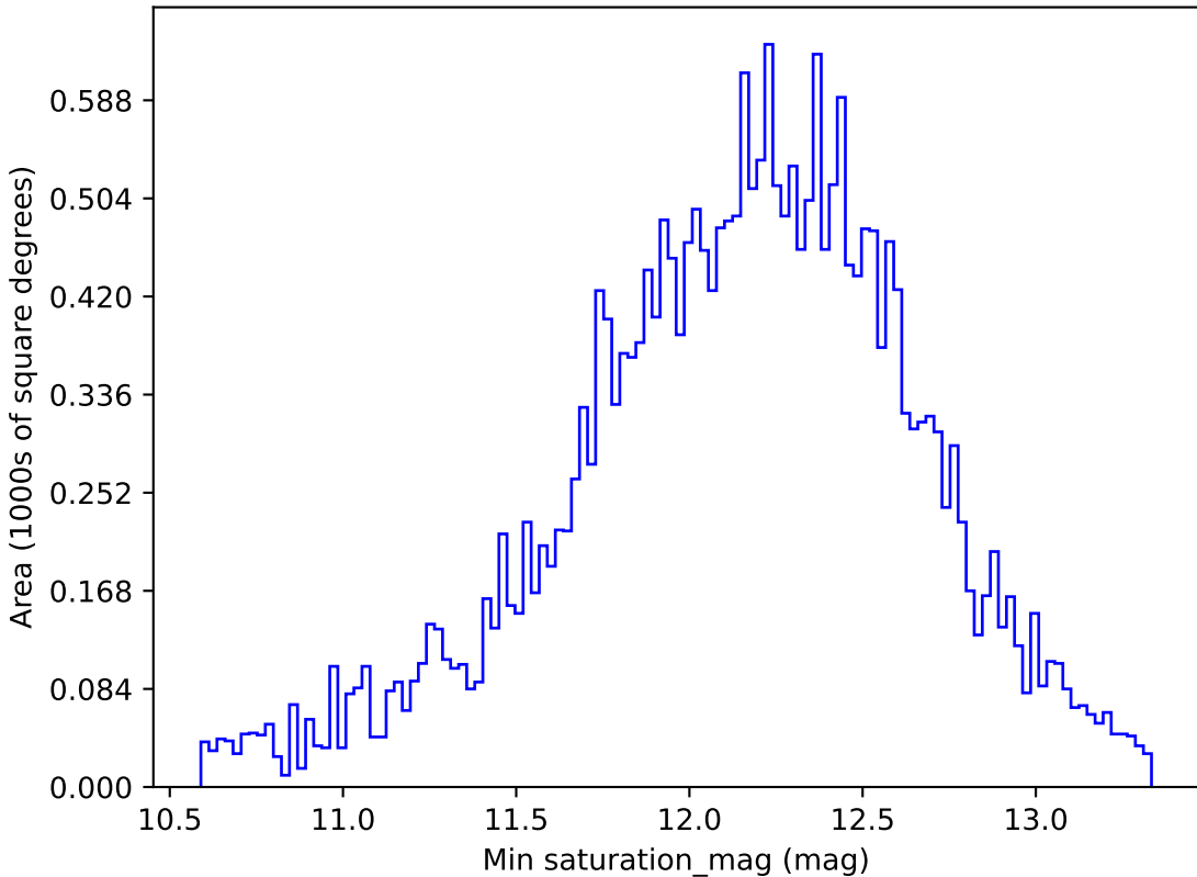
too_elab_r8_d2_gz_v3.4_10yrs All sky z band: Min saturation_mag
