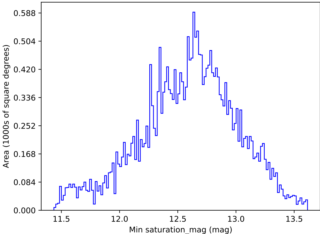
too_elab_r8_d2_gz_v3.4_10yrs All sky r band: Min saturation_mag
