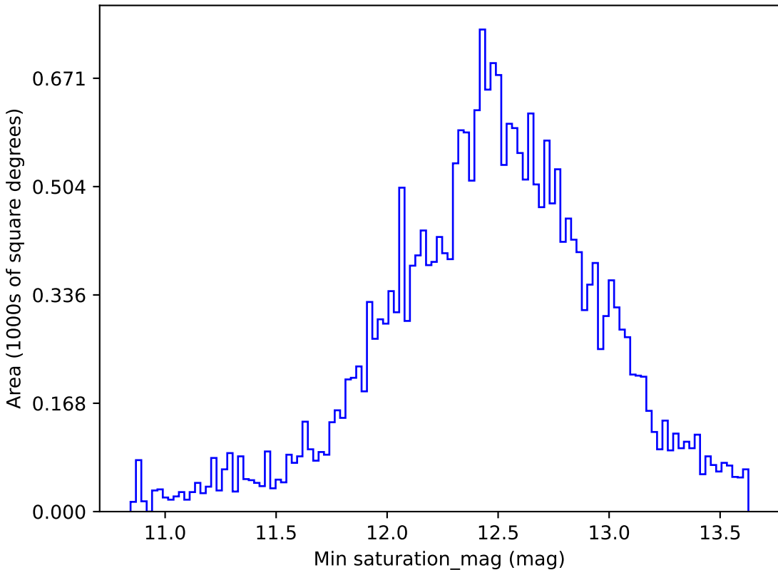
too_elab_r8_d2_gz_v3.4_10yrs All sky i band: Min saturation_mag
