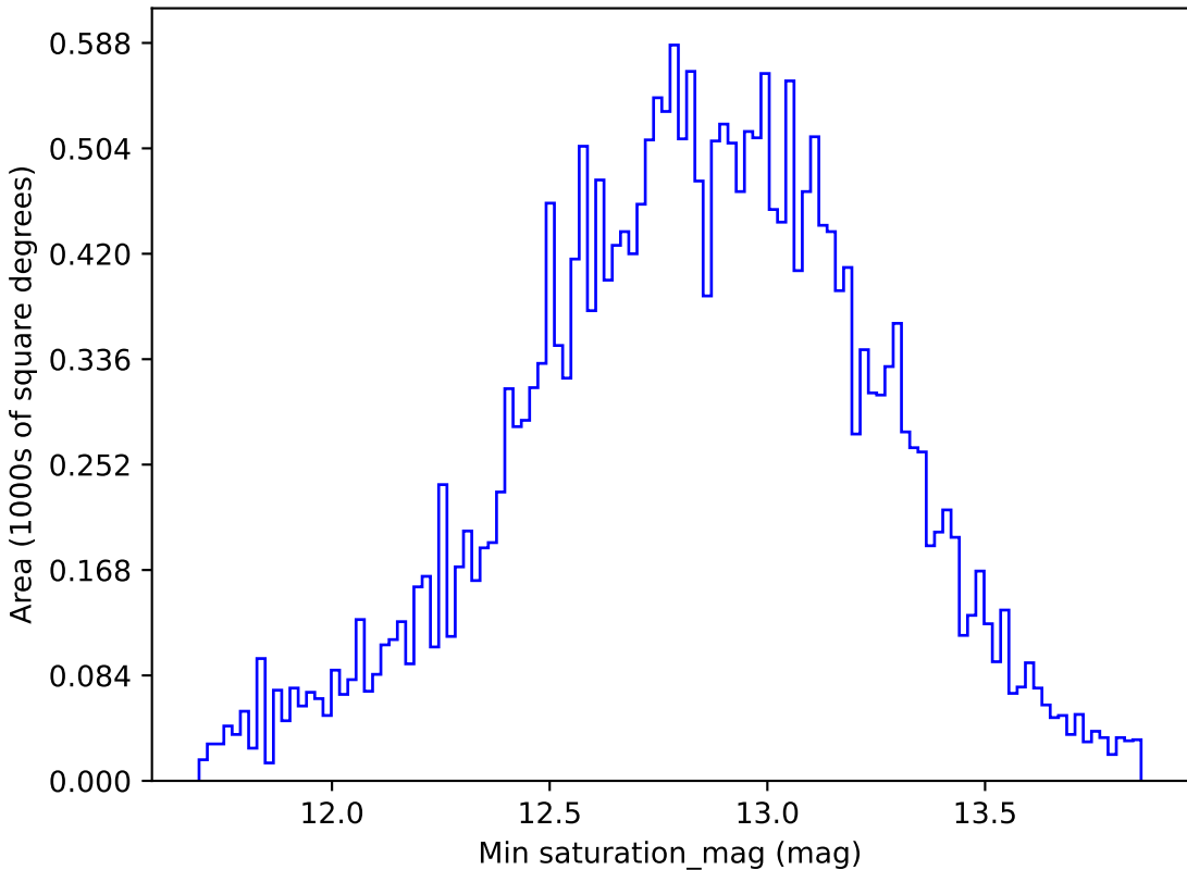
too_elab_r8_d2_gz_v3.4_10yrs All sky g band: Min saturation_mag
