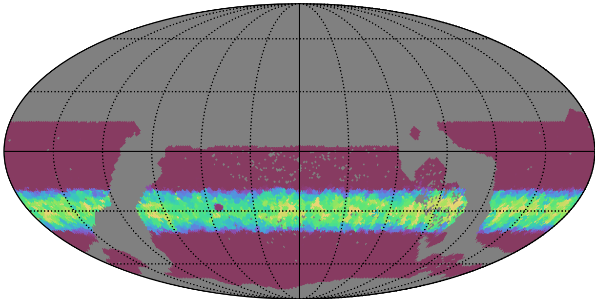
too_elab_r8_d2_gz_v3.4_10yrs WFD y band: Min normairmass
