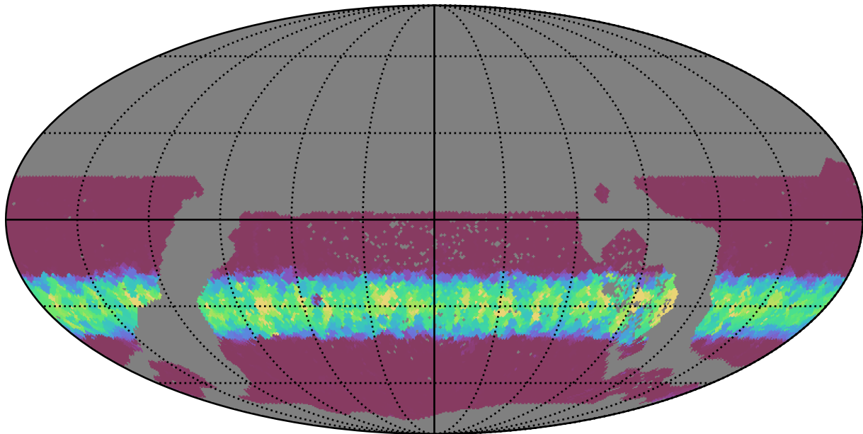
too_elab_r8_d2_gz_v3.4_10yrs WFD u band: Min normairmass
