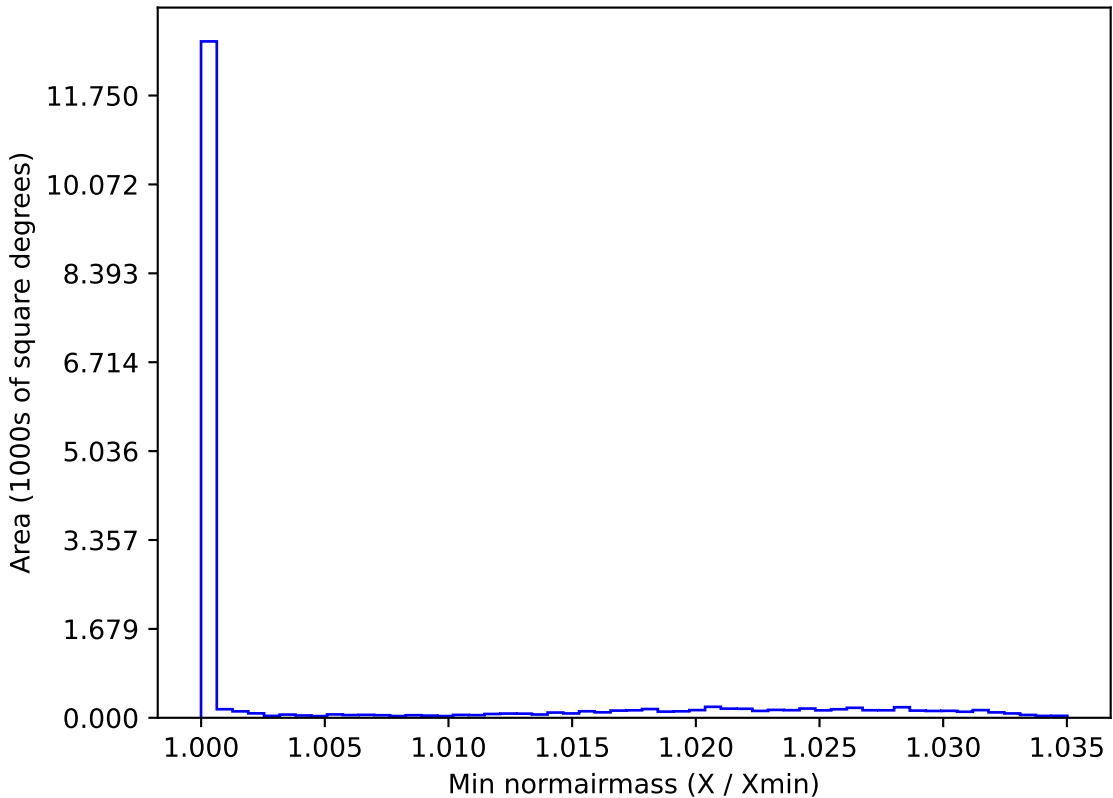
too_elab_r8_d2_gz_v3.4_10yrs WFD r band: Min normairmass
