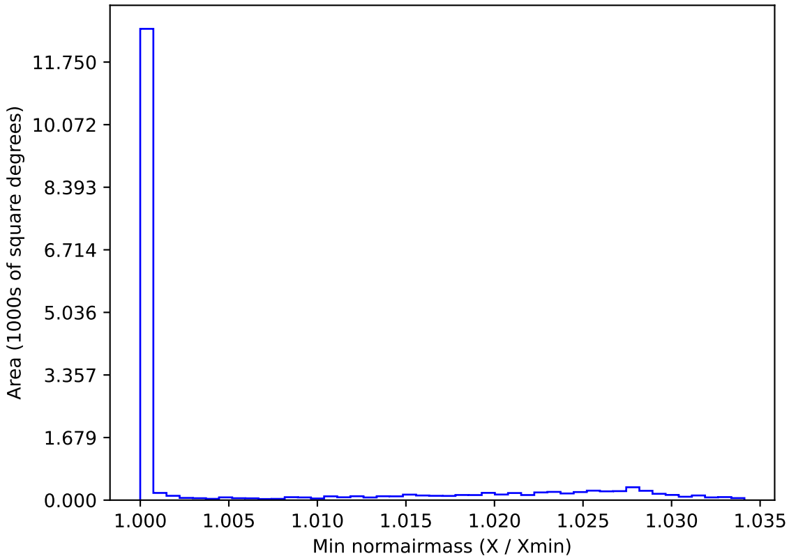
too_elab_r8_d2_gz_v3.4_10yrs WFD i band: Min normairmass
