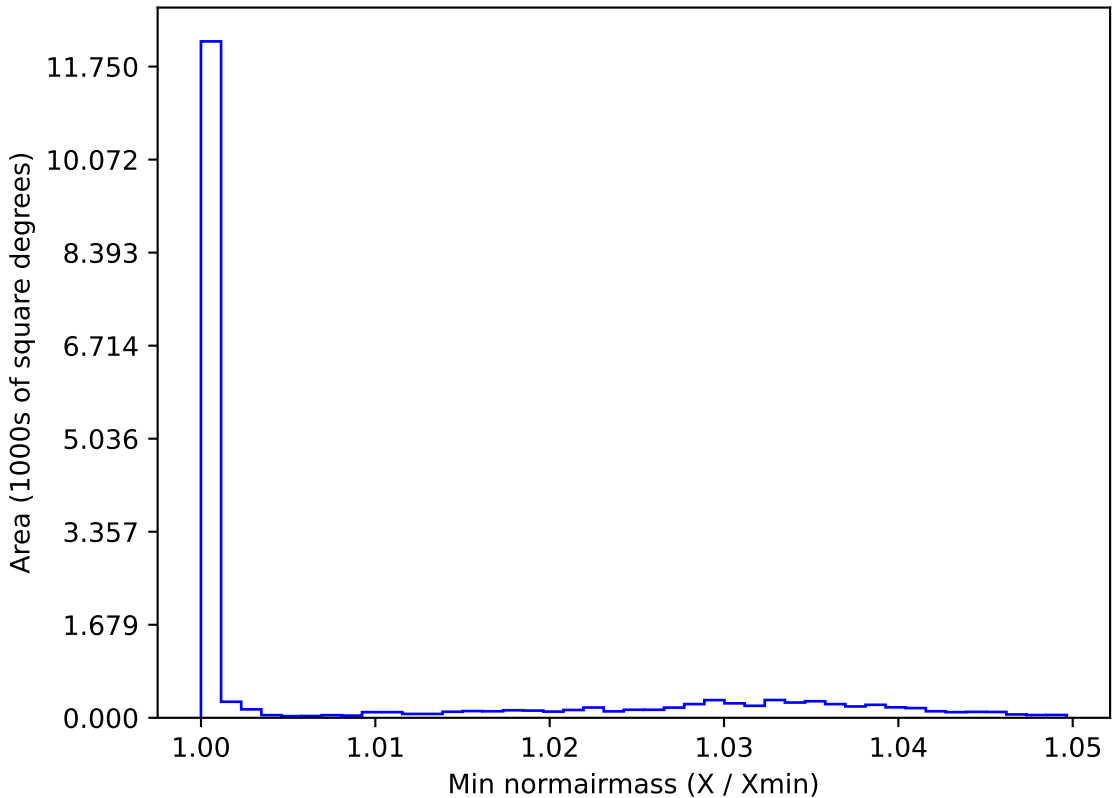
too_elab_r8_d2_gz_v3.4_10yrs WFD g band: Min normairmass
