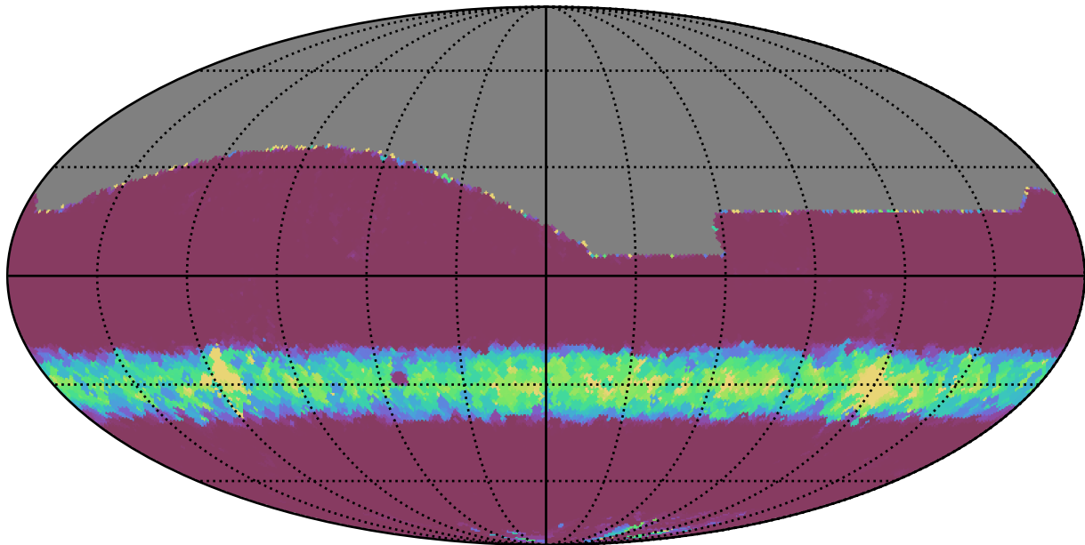
too_elab_r8_d2_gz_v3.4_10yrs All sky r band: Min normairmass
