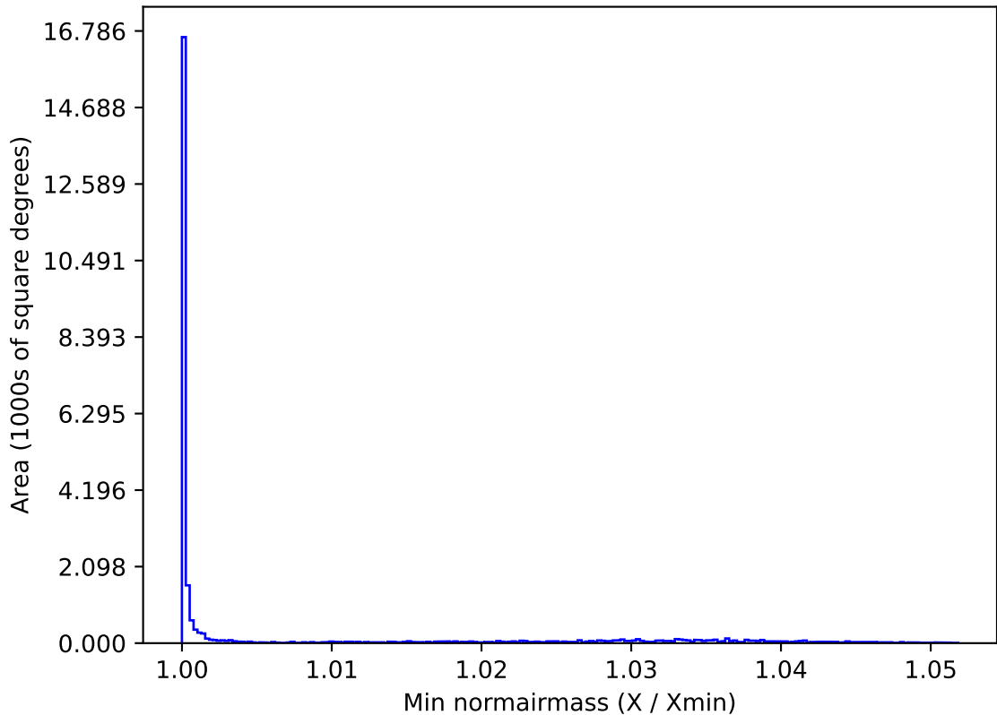
too_elab_r8_d2_gz_v3.4_10yrs All sky g band: Min normairmass
