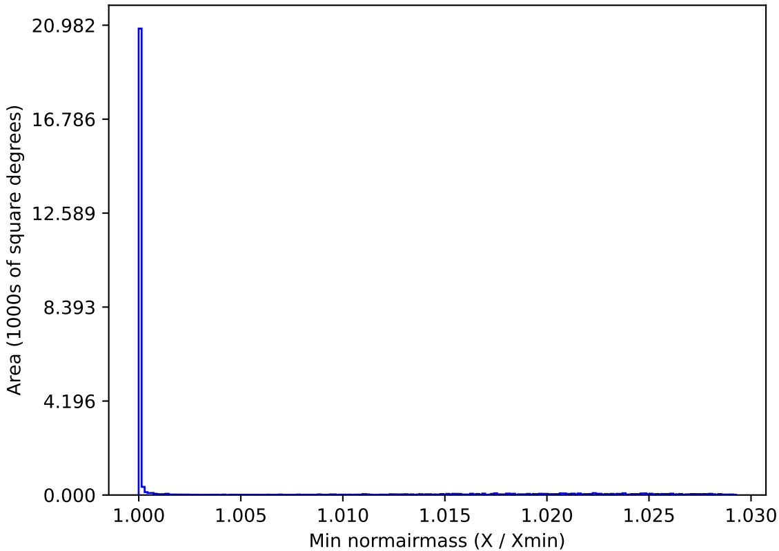
too_elab_r8_d2_gz_v3.4_10yrs All sky all bands: Min normairmass
