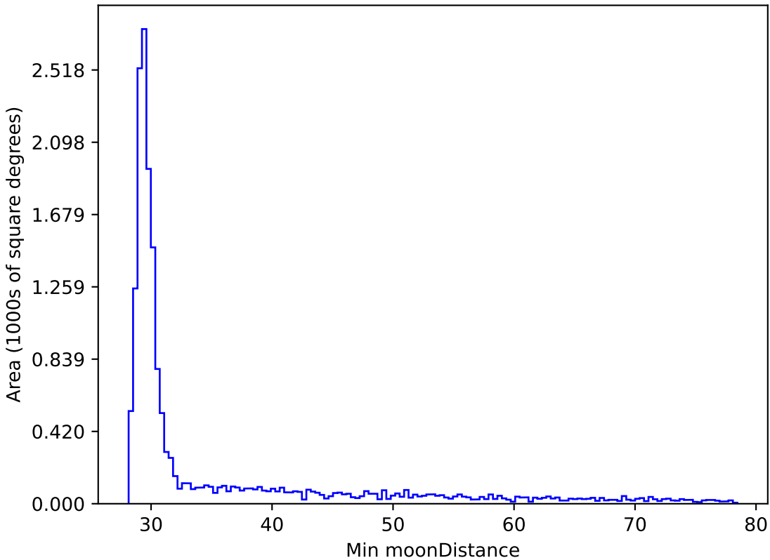
too_elab_r8_d2_gz_v3.4_10yrs WFD y band: Min moonDistance
