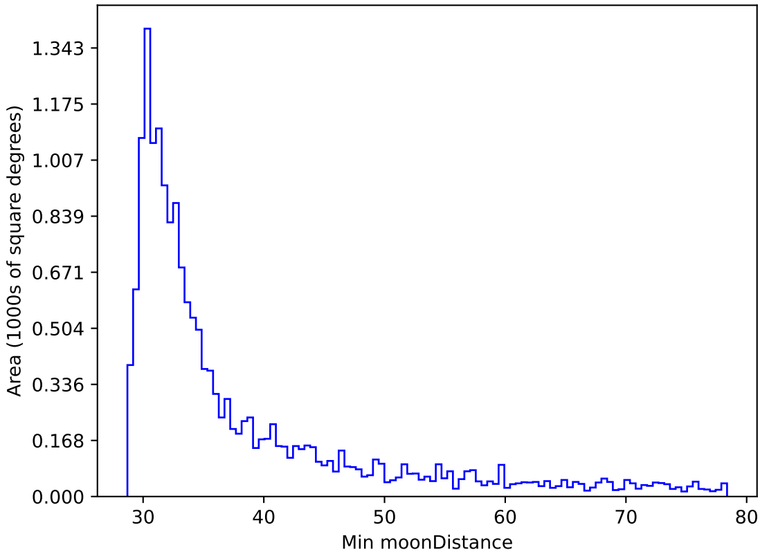
too_elab_r8_d2_gz_v3.4_10yrs WFD r band: Min moonDistance
