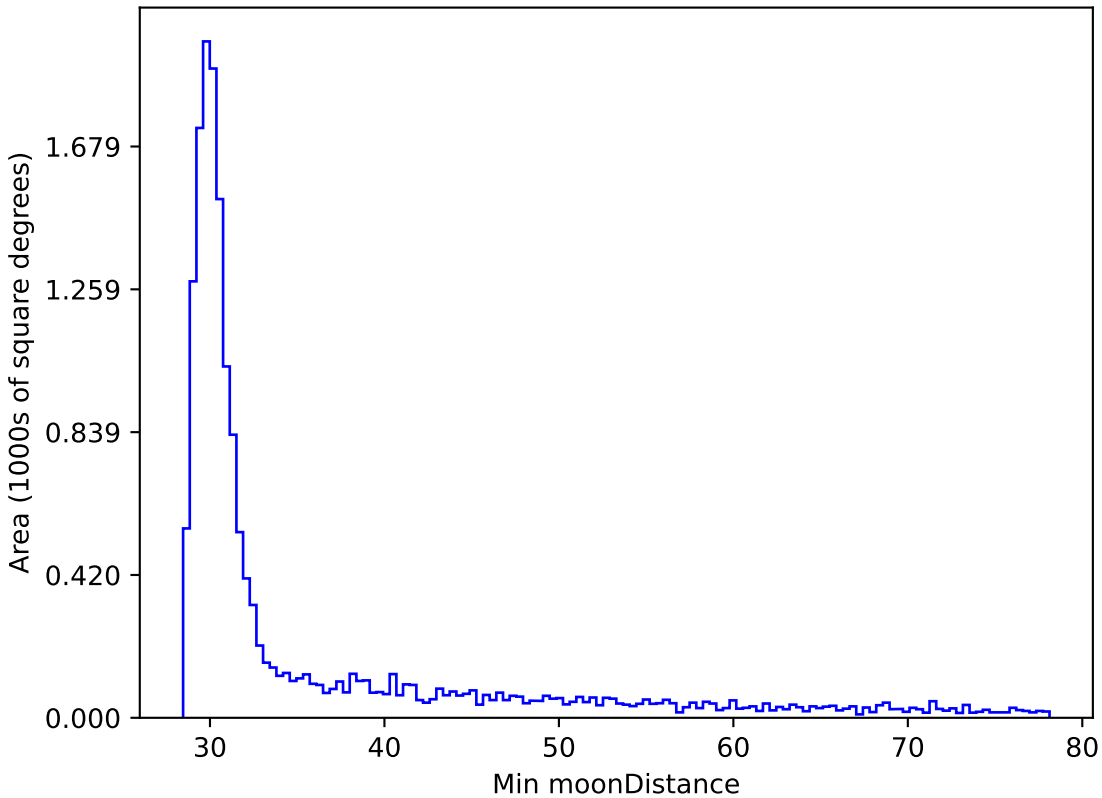
too_elab_r8_d2_gz_v3.4_10yrs WFD i band: Min moonDistance
