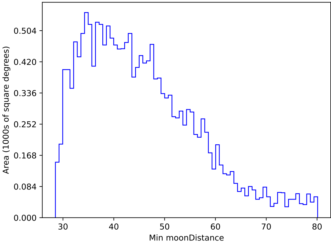
too_elab_r8_d2_gz_v3.4_10yrs WFD g band: Min moonDistance
