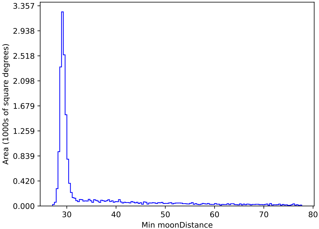
too_elab_r8_d2_gz_v3.4_10yrs WFD all bands: Min moonDistance
