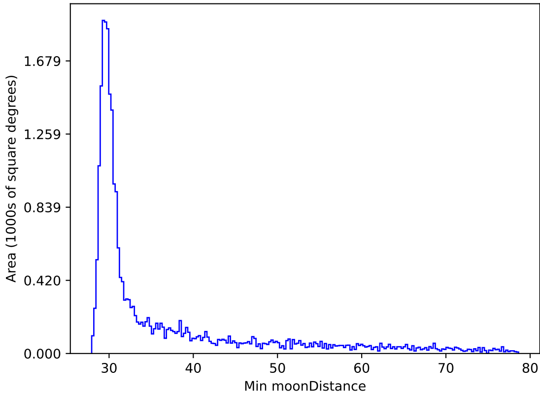
too_elab_r8_d2_gz_v3.4_10yrs All sky z band: Min moonDistance
