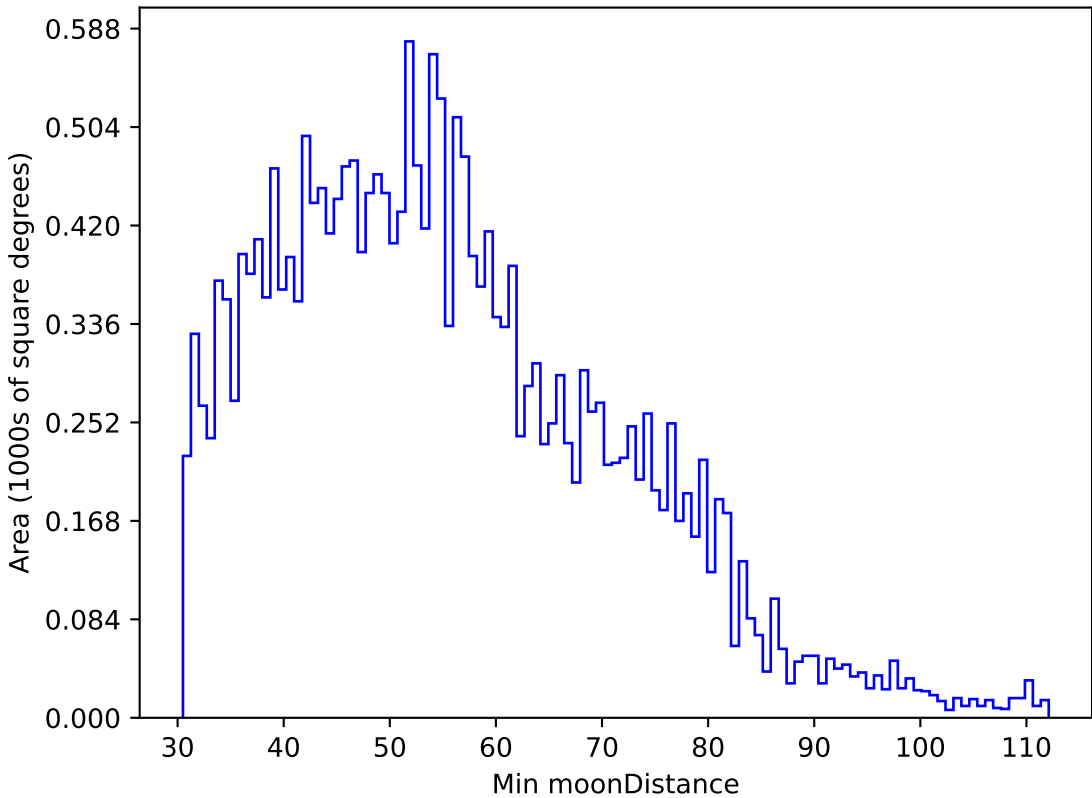
too_elab_r8_d2_gz_v3.4_10yrs All sky u band: Min moonDistance
