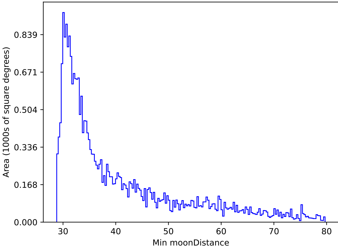
too_elab_r8_d2_gz_v3.4_10yrs All sky r band: Min moonDistance
