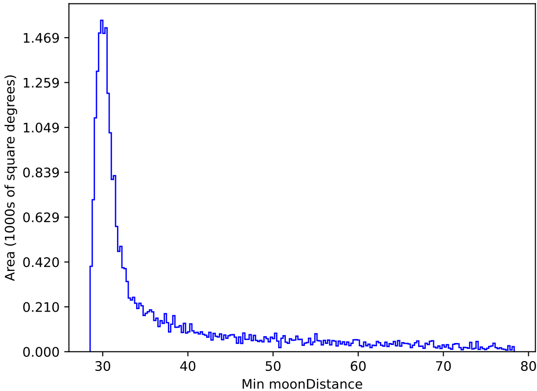
too_elab_r8_d2_gz_v3.4_10yrs All sky i band: Min moonDistance
