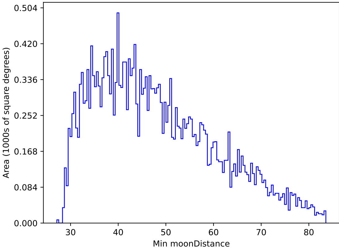
too_elab_r8_d2_gz_v3.4_10yrs All sky g band: Min moonDistance
