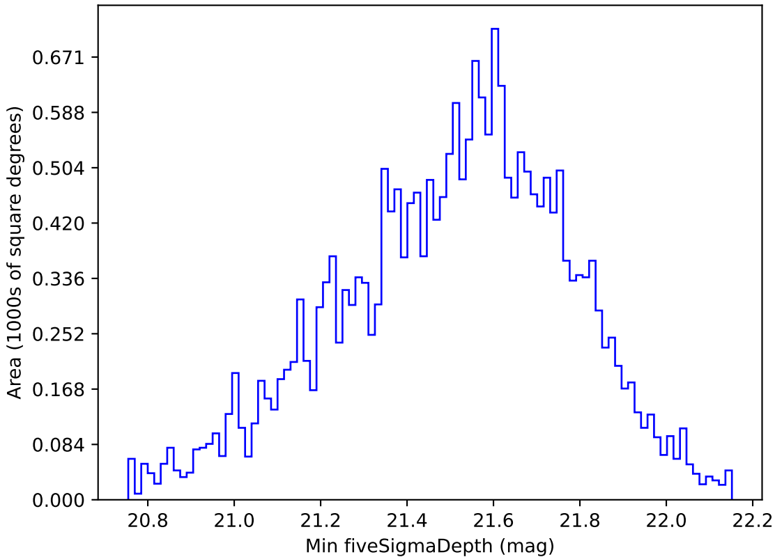
too_elab_r8_d2_gz_v3.4_10yrs Yr 1 y band: Min fiveSigmaDepth
