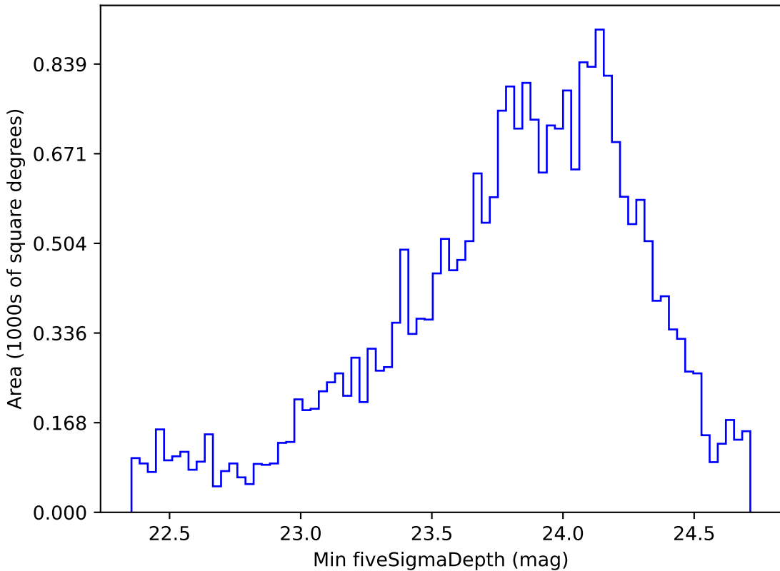
too_elab_r8_d2_gz_v3.4_10yrs Yr 1 g band: Min fiveSigmaDepth
