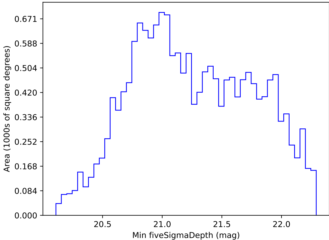
too_elab_r8_d2_gz_v3.4_10yrs WFD z band: Min fiveSigmaDepth
