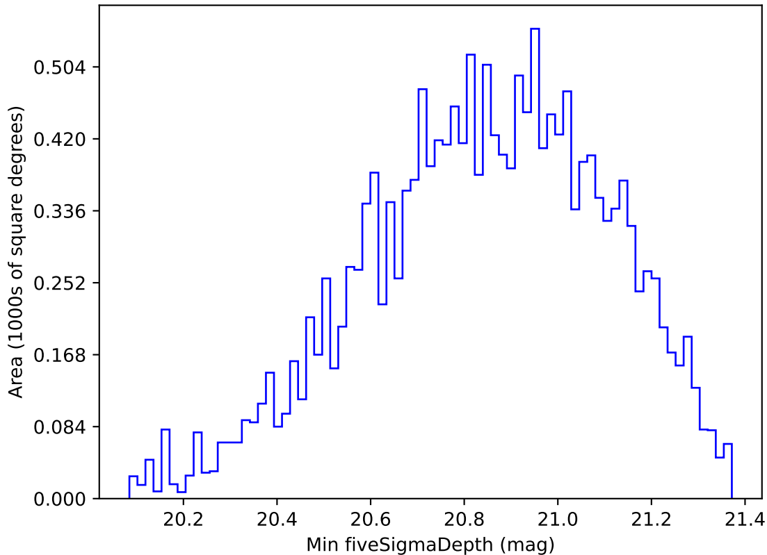
too_elab_r8_d2_gz_v3.4_10yrs WFD y band: Min fiveSigmaDepth
