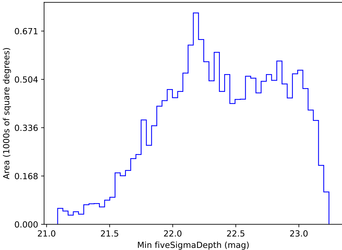
too_elab_r8_d2_gz_v3.4_10yrs WFD r band: Min fiveSigmaDepth
