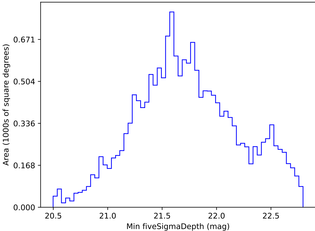
too_elab_r8_d2_gz_v3.4_10yrs WFD i band: Min fiveSigmaDepth
