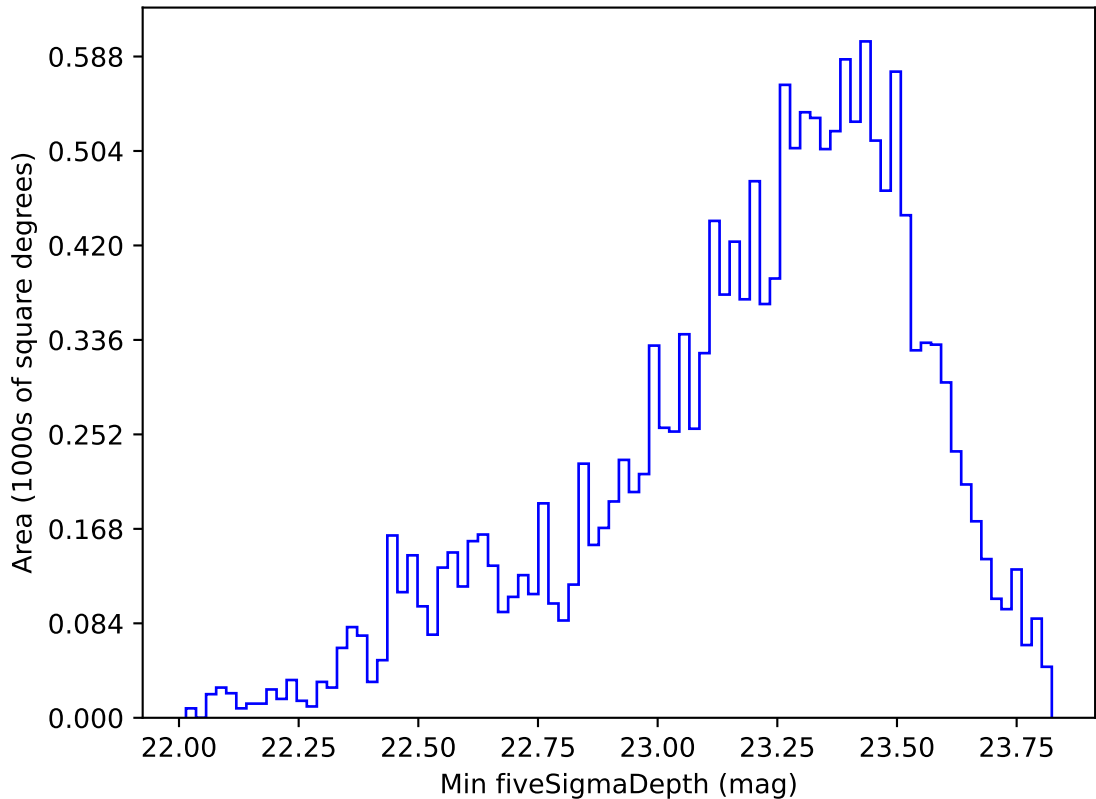
too_elab_r8_d2_gz_v3.4_10yrs WFD g band: Min fiveSigmaDepth
