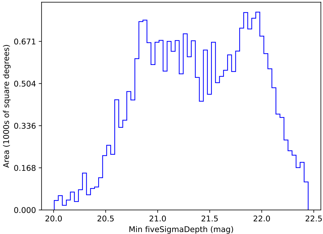
too_elab_r8_d2_gz_v3.4_10yrs All sky z band: Min fiveSigmaDepth
