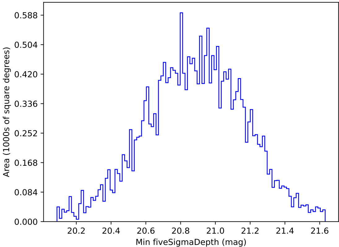
too_elab_r8_d2_gz_v3.4_10yrs All sky y band: Min fiveSigmaDepth
