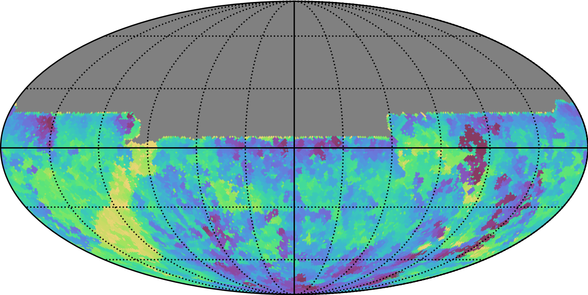
too_elab_r8_d2_gz_v3.4_10yrs All sky u band: Min fiveSigmaDepth
