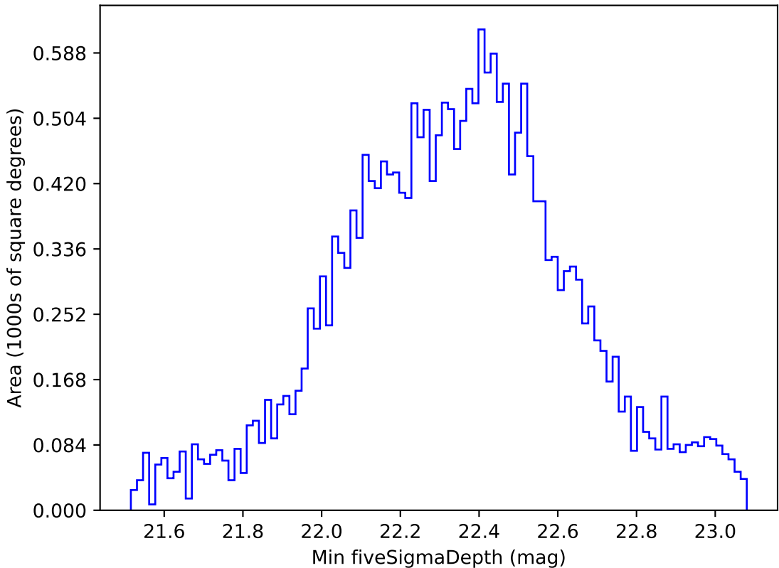
too_elab_r8_d2_gz_v3.4_10yrs All sky u band: Min fiveSigmaDepth
