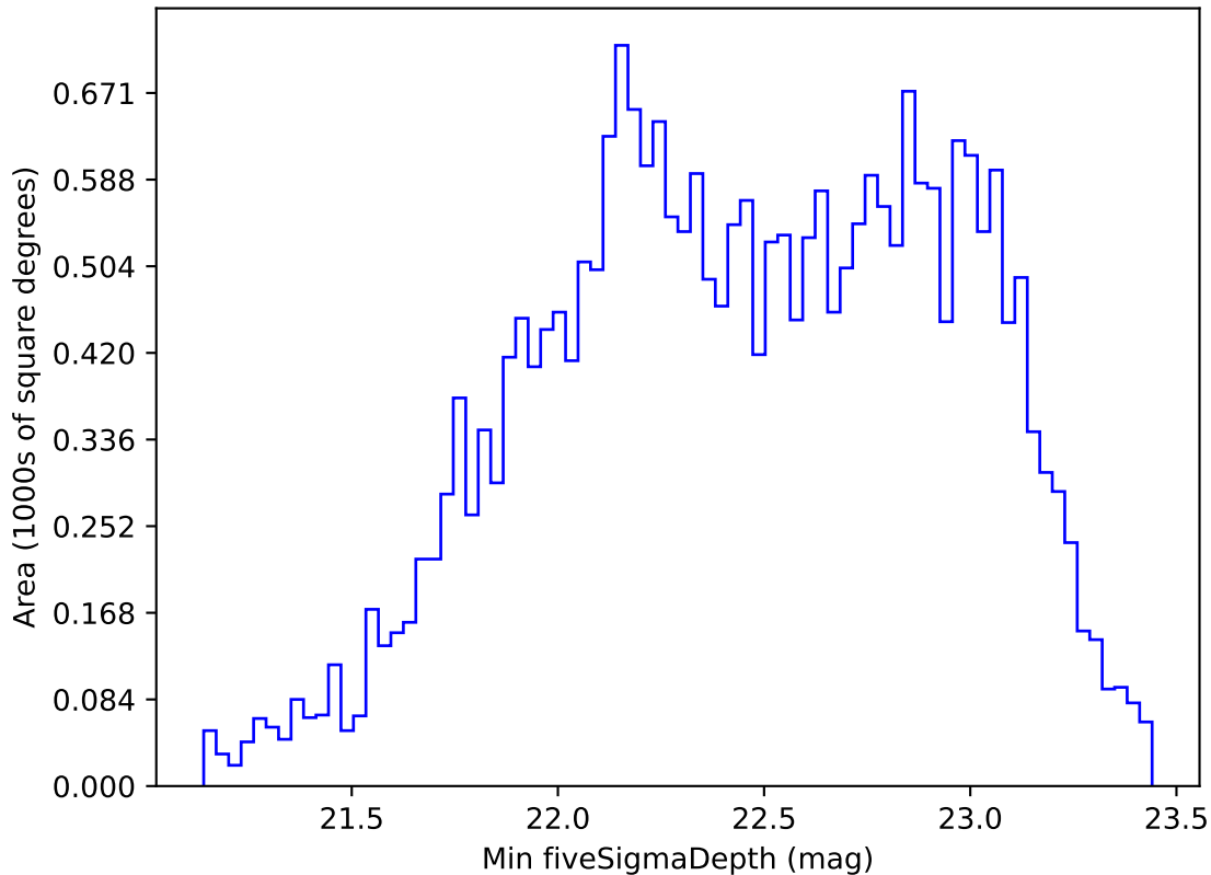
too_elab_r8_d2_gz_v3.4_10yrs All sky r band: Min fiveSigmaDepth
