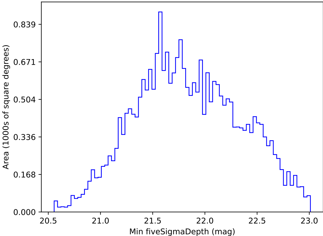
too_elab_r8_d2_gz_v3.4_10yrs All sky i band: Min fiveSigmaDepth
