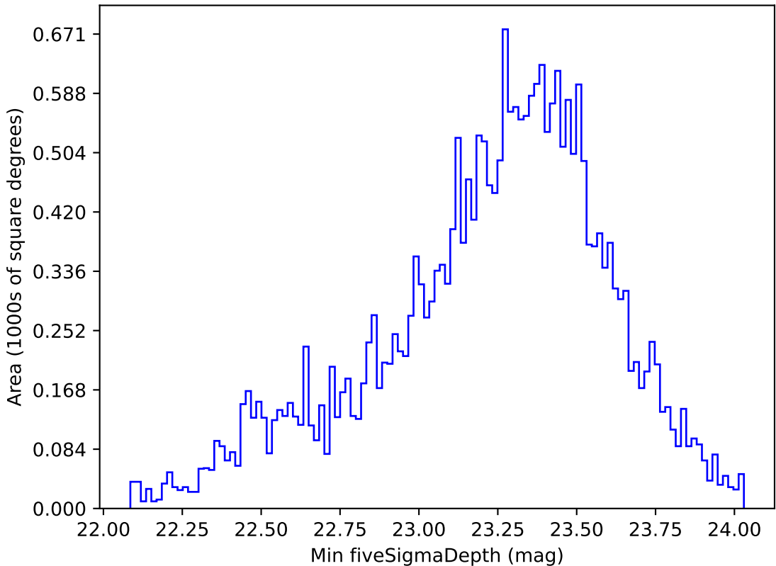
too_elab_r8_d2_gz_v3.4_10yrs All sky g band: Min fiveSigmaDepth
